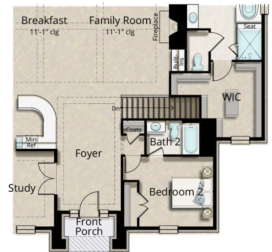
First Floor Stairs to Optional Basement
